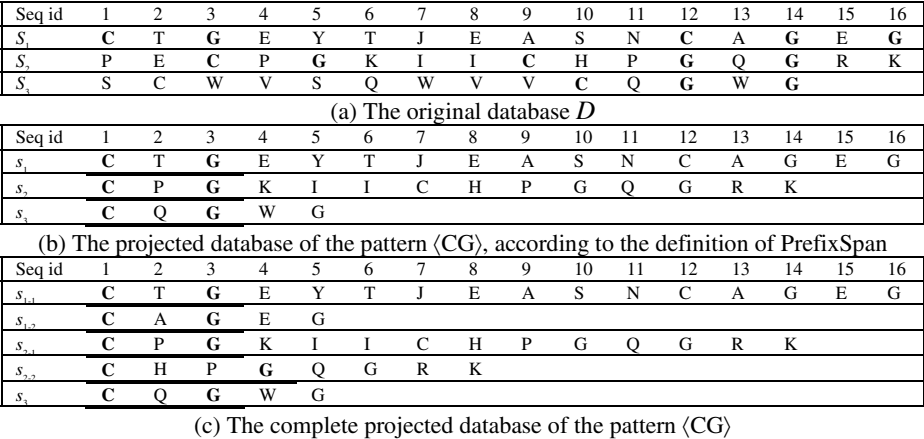
Fig. 1. Illustration of the complete projected database
