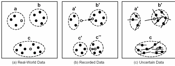
Fig. 1. (a) The real-world data are partitioned into three clusters (a, b, c). (b) The recorded locations of some objects (shaded) are not the same as their true location, thus creating clusters a' , b' , c' and c'' . (c) When line uncertainty is considered, clusters a' , b' and c are produced. The clustering result is closer to that of (a) than (b) is.
