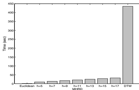
Fig. 7. Time performances of the methods in the experiment
