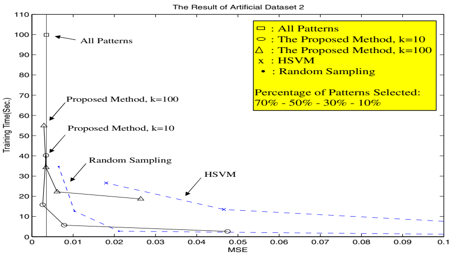
Fig. 8. The Result of Artificial Dataset 2 ( c=4.6723 , \varepsilon=0.1643 )
