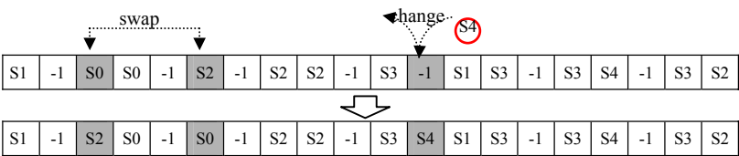
Fig. 4. mutation
