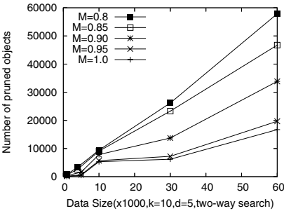
Fig. 9. Pruning results (1)
