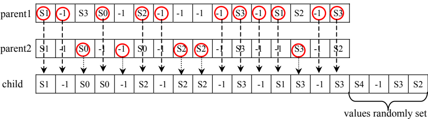
Fig. 3. crossover
