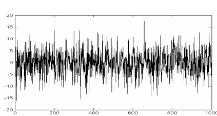
Fig. 5. White Noise WN(0,0.5)
