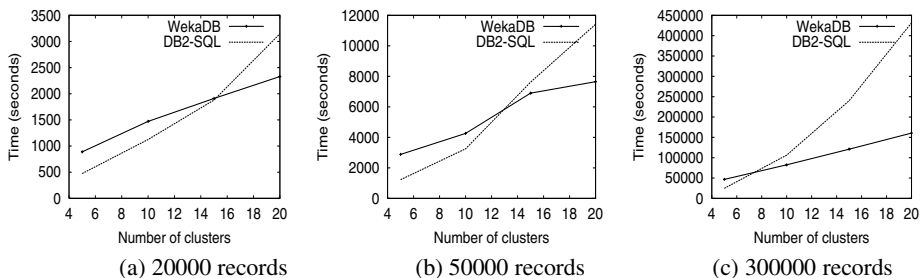
Fig. 5. DB-SQL and buffered WekaDB for k-means clustering on different dataset sizes (synthetic data)
