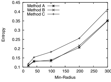
Fig. 7. Synthetic Data(1)
