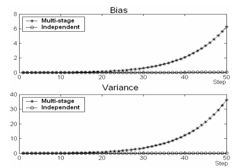
Fig. 3. Bias and variance for HMM/MLR
