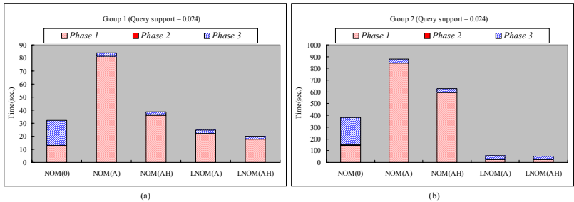
Fig. 2. Execution times spent by the NOM and LNOP algorithms on Groups 1 to 2
