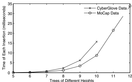
Fig. 10. Time taken for inserting a new motion ID in the indexing tree
