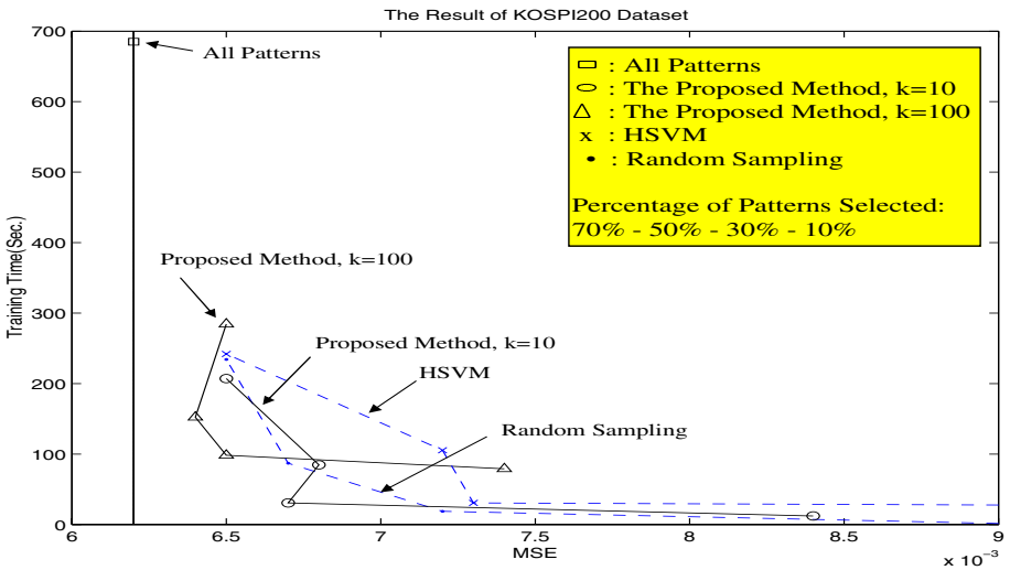
Fig. 10. The Result of KOSPI200 Dataset ( c=3.3112 , \varepsilon=0.0631 )
