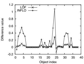
Fig. 6. LOF and INFLO
