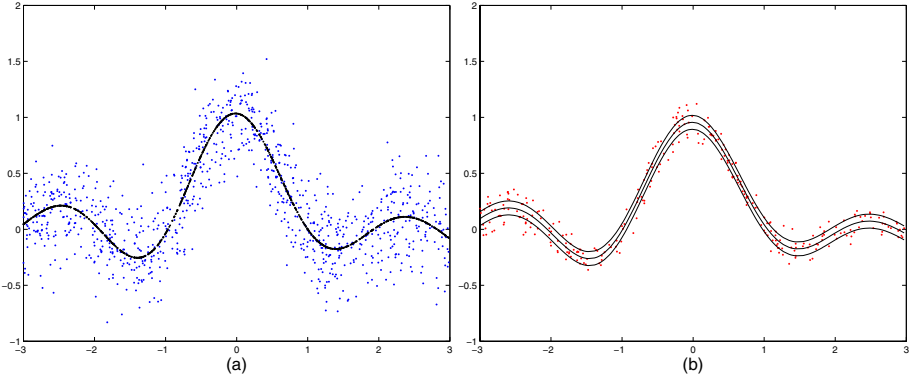
Fig. 2. (a) The regression function after training original pattern set, and (b) The regression function after training ONLY patterns inside estimated \varepsilon -tube
