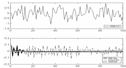
Fig. 6. Predicting Results ( p=12, h=100, d=6 )
