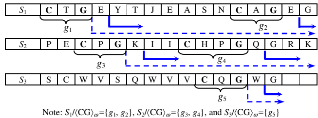
Fig. 2. The scenario of scanning a projected database
