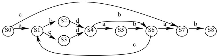
Fig. 1. a finite state automaton
