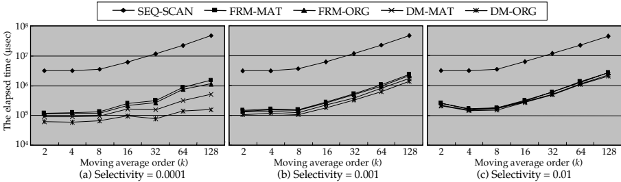
Fig. 3. The elapsed times for STOCK-DATA on different selectivities
