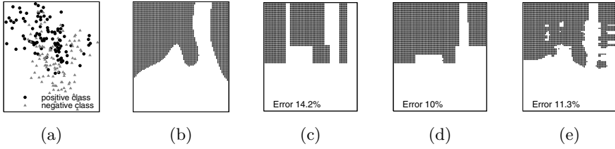
Fig. 1. Gaussian mixture (a) training data and (b) the optimal boundary. Shaded area denotes positive class; cleared area denotes negative class. (c) When classifying using a single unpruned decision tree, C4.5, the decision boundary is rectangular in shape. (d) The decision boundary of Random Forests ( F = 1 ) retains the rectangularity from the single decision tree. (e) Max-diverse Ensemble fits a non-axis-parallel decision boundary to the training data, forming non-rectangular boundaries.
