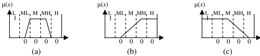
Fig. 1. Examples of an antecedent fuzzy set A_{ji} with linguistic values (L: low, ML: medium low, M: medium, MH: medium high, H: high). (a) A_{ji} represents \{ML, M, MH\} . (b) A_{ji} represents \{ML, M, MH, H\} , i.e., not Low. (c) A_{ji} represents \{L, ML, M, MH, H\} or ALL.
