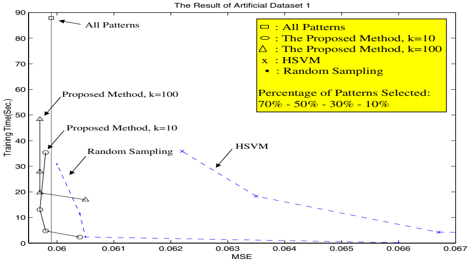
Fig. 7. The Result of Artificial Dataset 1 ( c=1.5058 , \varepsilon=0.1247 )
