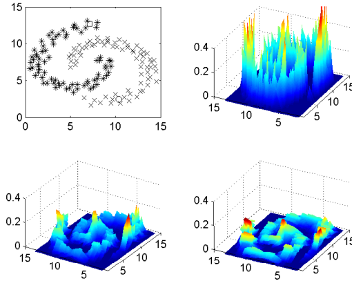
Fig. 1. Smooth graph on artificial data. \sigma = 0.45 . Right up: m = 1 ; Left bottom: m = 5 ; Right bottom: m = 9
