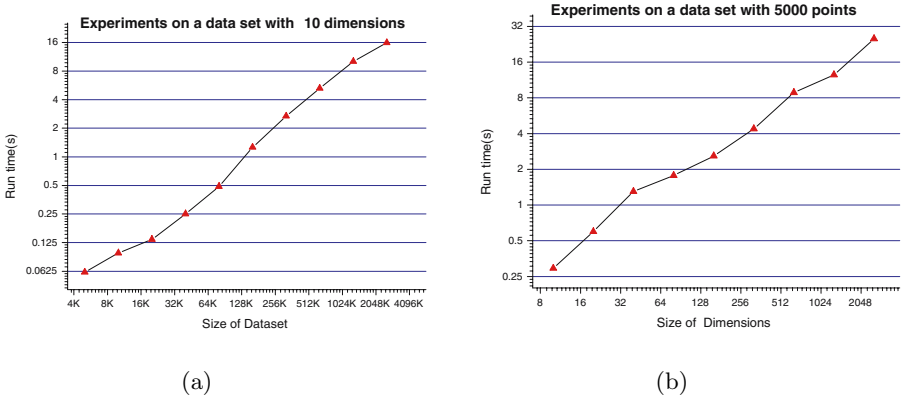
Fig. 3. Scalability against the data size and dimensions
