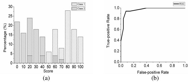
Fig. 3. The (a) score distribution histogram and (b) ROC curve of data set prostate in one run of 10-CV. The test accuracy and AUC are 93.00% and 0.963.
