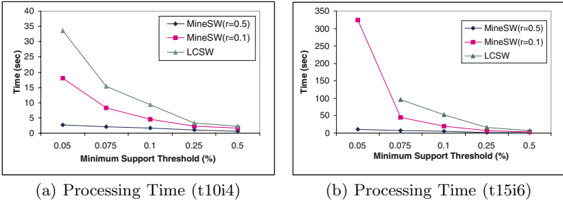
Fig. 2. Processing Time with Varying Minimum Support Threshold
